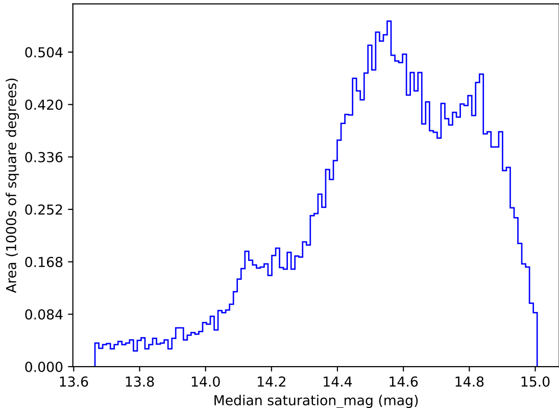
no_magell_roll_v3.4_10yrs All sky r band: Median saturation_mag
