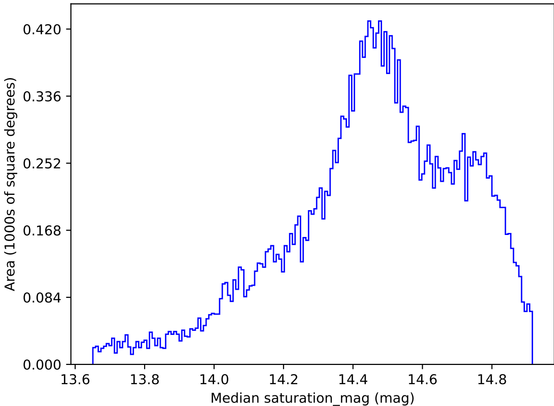
no_magell_roll_v3.4_10yrs All sky i band: Median saturation_mag
