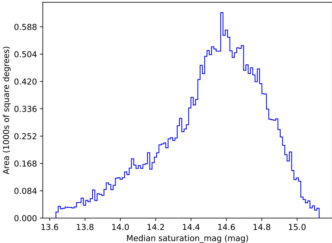
no_magell_roll_v3.4_10yrs All sky g band: Median saturation_mag
