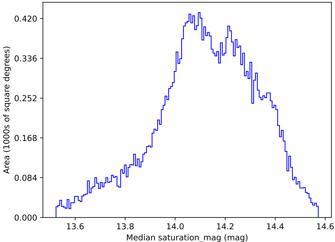
no_magell_roll_v3.4_10yrs All sky all bands: Median saturation_mag
