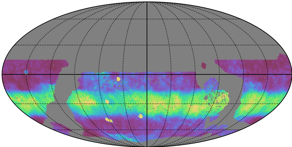
no_magell_roll_v3.4_10yrs WFD z band: Median normairmass
