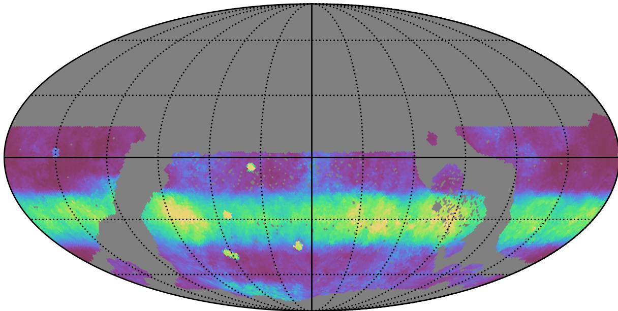
no_magell_roll_v3.4_10yrs WFD r band: Median normairmass
