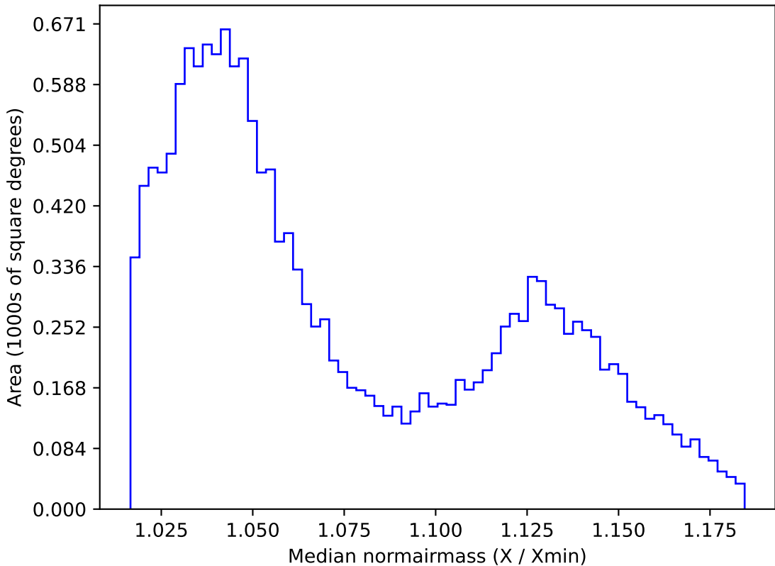
no_magell_roll_v3.4_10yrs WFD r band: Median normairmass
