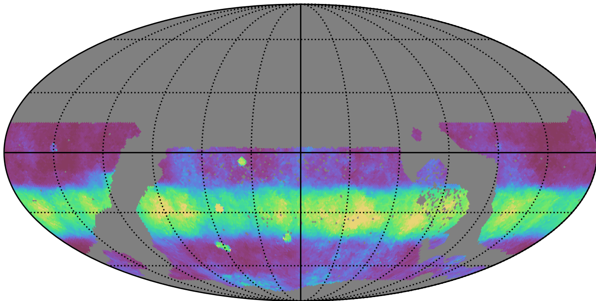
no_magell_roll_v3.4_10yrs WFD i band: Median normairmass
