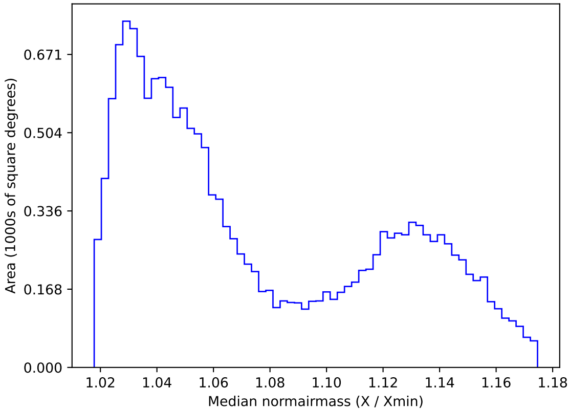
no_magell_roll_v3.4_10yrs WFD i band: Median normairmass
