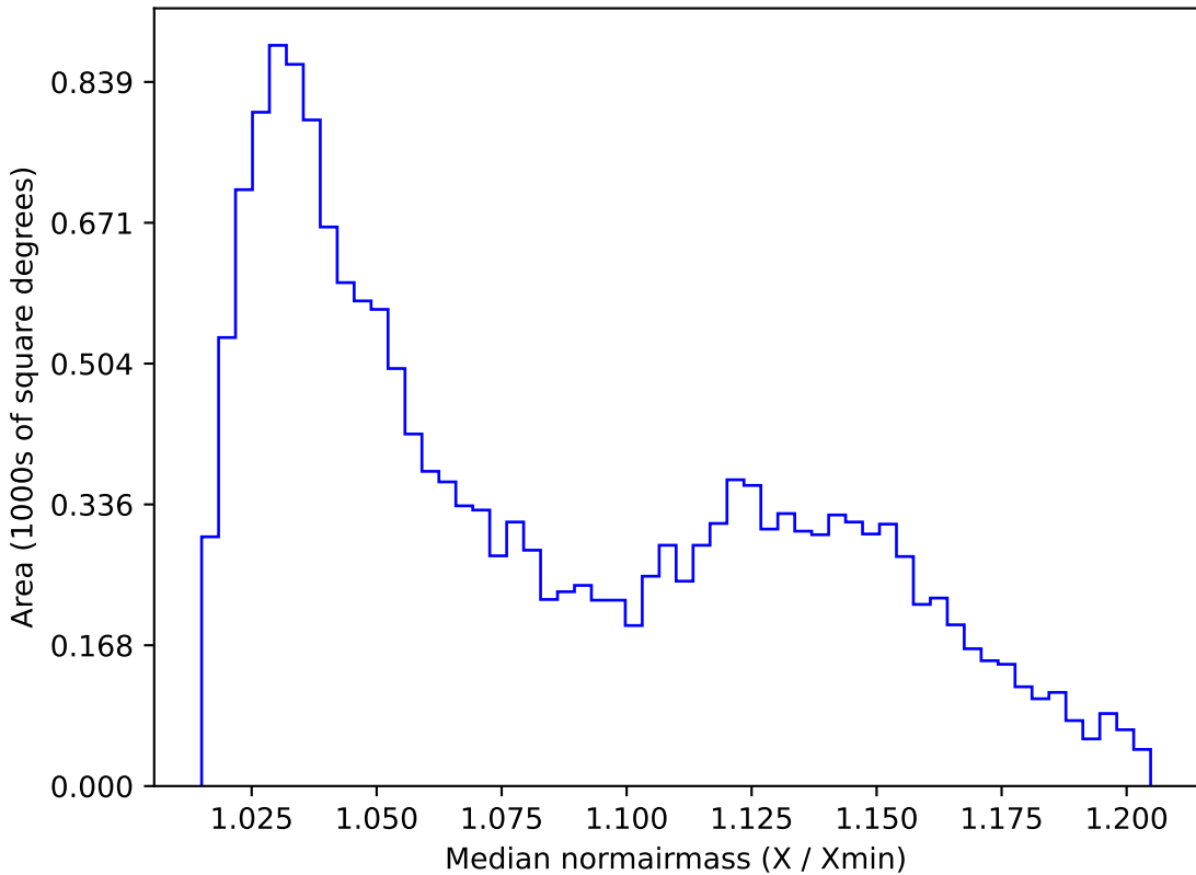
no_magell_roll_v3.4_10yrs WFD g band: Median normairmass
