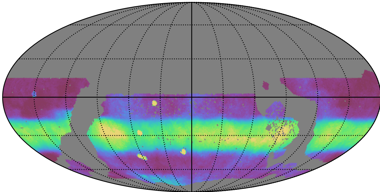
no_magell_roll_v3.4_10yrs WFD all bands: Median normairmass
