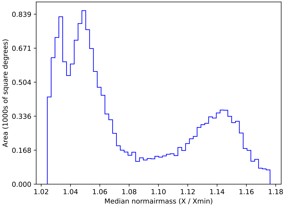
no_magell_roll_v3.4_10yrs WFD all bands: Median normairmass
