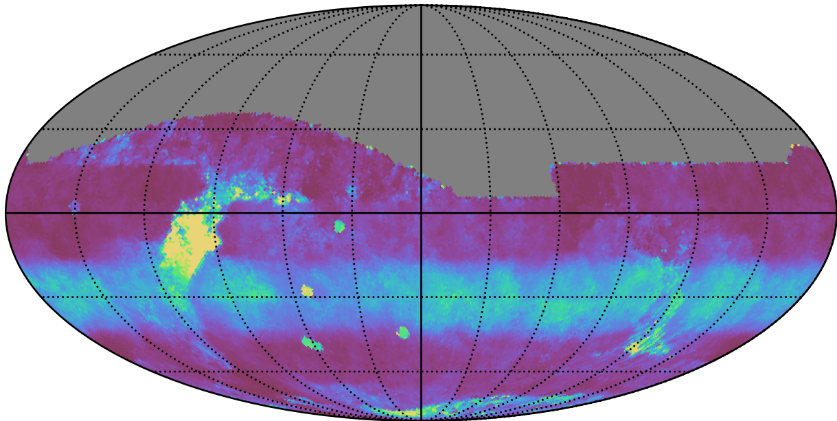
no_magell_roll_v3.4_10yrs All sky z band: Median normairmass
