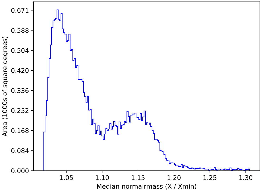
no_magell_roll_v3.4_10yrs All sky z band: Median normairmass
