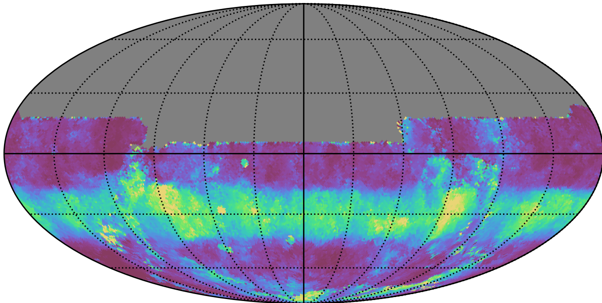
no_magell_roll_v3.4_10yrs All sky u band: Median normairmass
