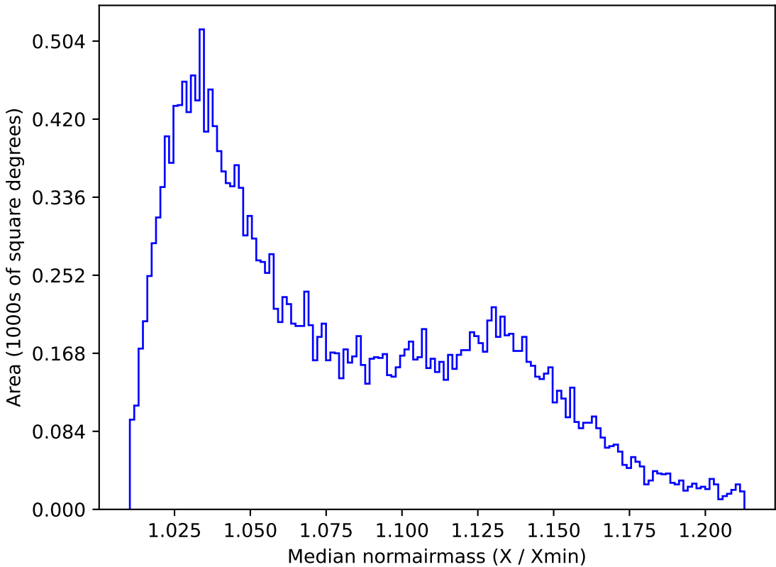
no_magell_roll_v3.4_10yrs All sky u band: Median normairmass
