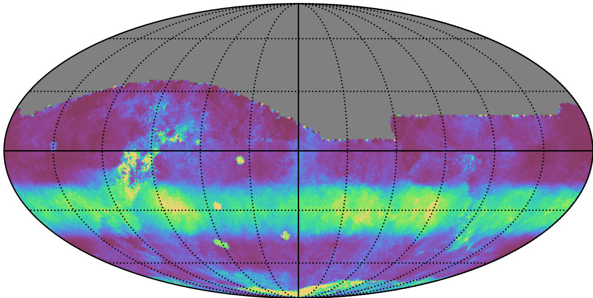
no_magell_roll_v3.4_10yrs All sky r band: Median normairmass
