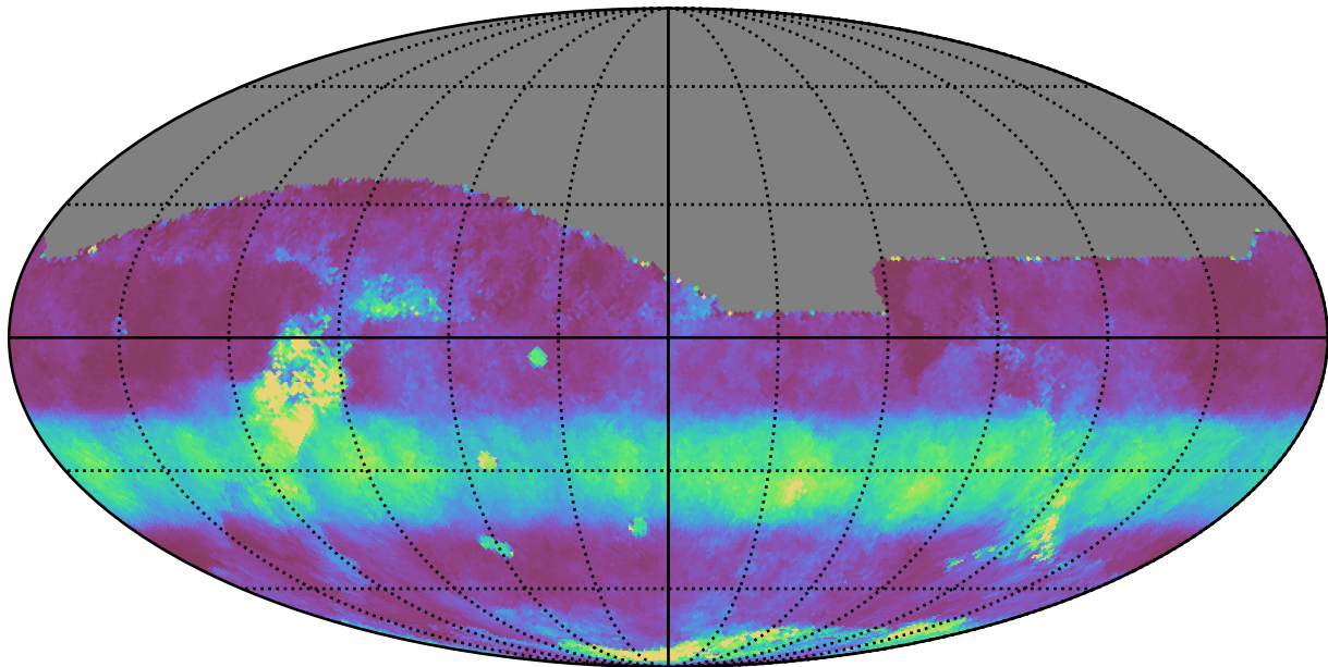
no_magell_roll_v3.4_10yrs All sky i band: Median normairmass
