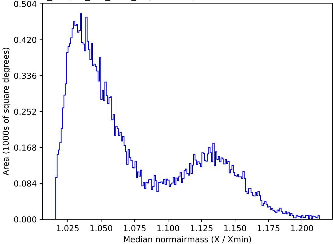
no_magell_roll_v3.4_10yrs All sky i band: Median normairmass
