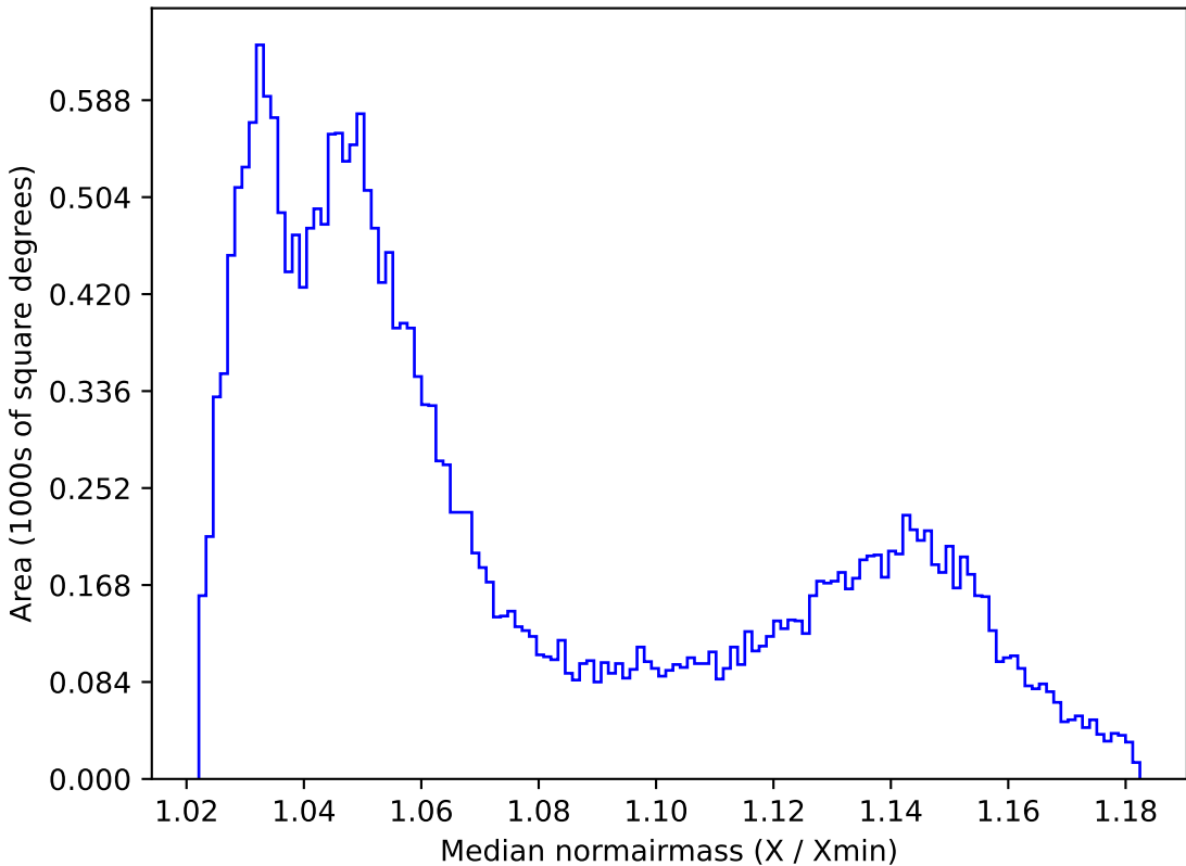
no_magell_roll_v3.4_10yrs All sky all bands: Median normairmass
