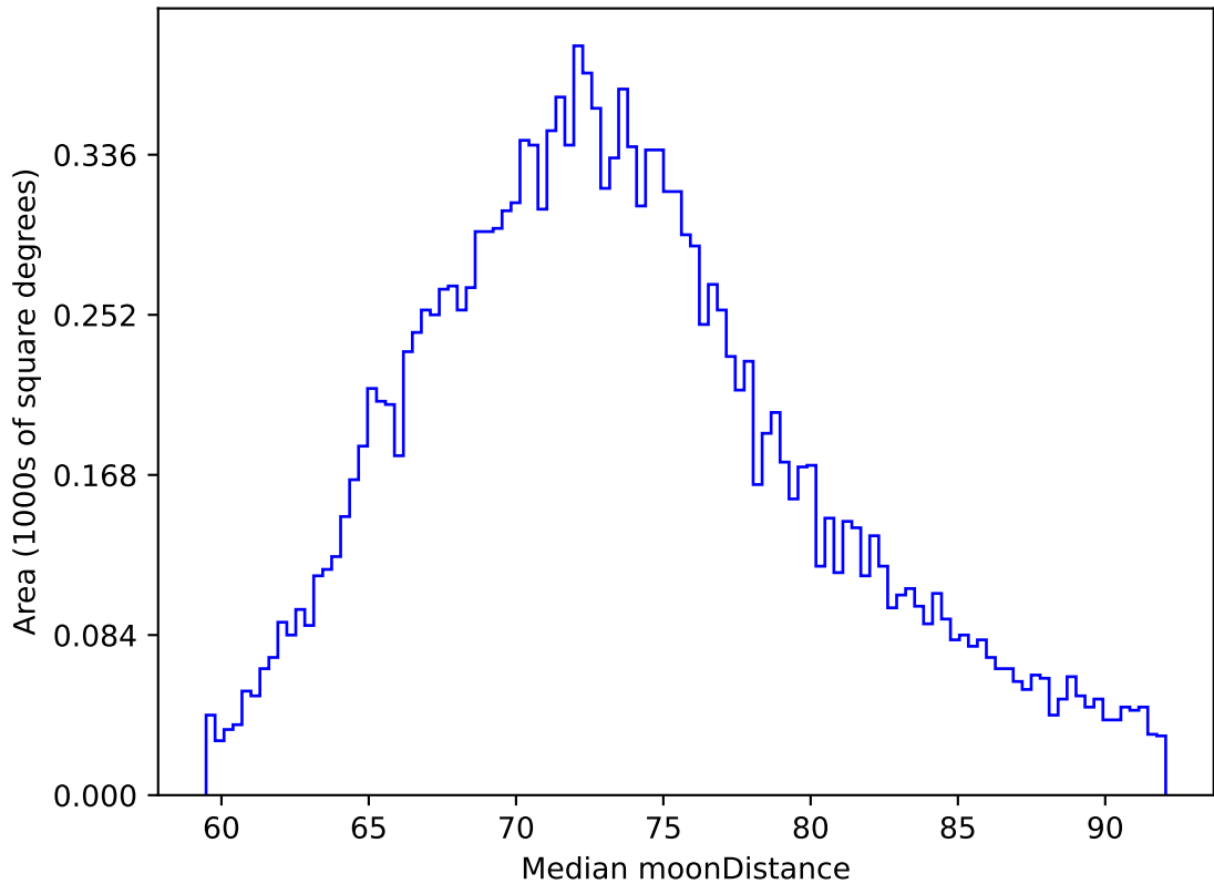
no_magell_roll_v3.4_10yrs WFD z band: Median moonDistance
