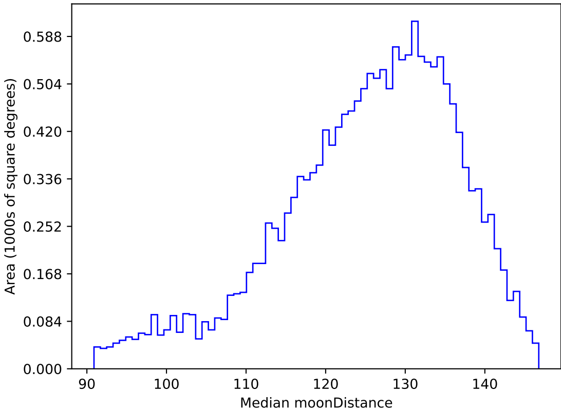
no_magell_roll_v3.4_10yrs WFD u band: Median moonDistance
