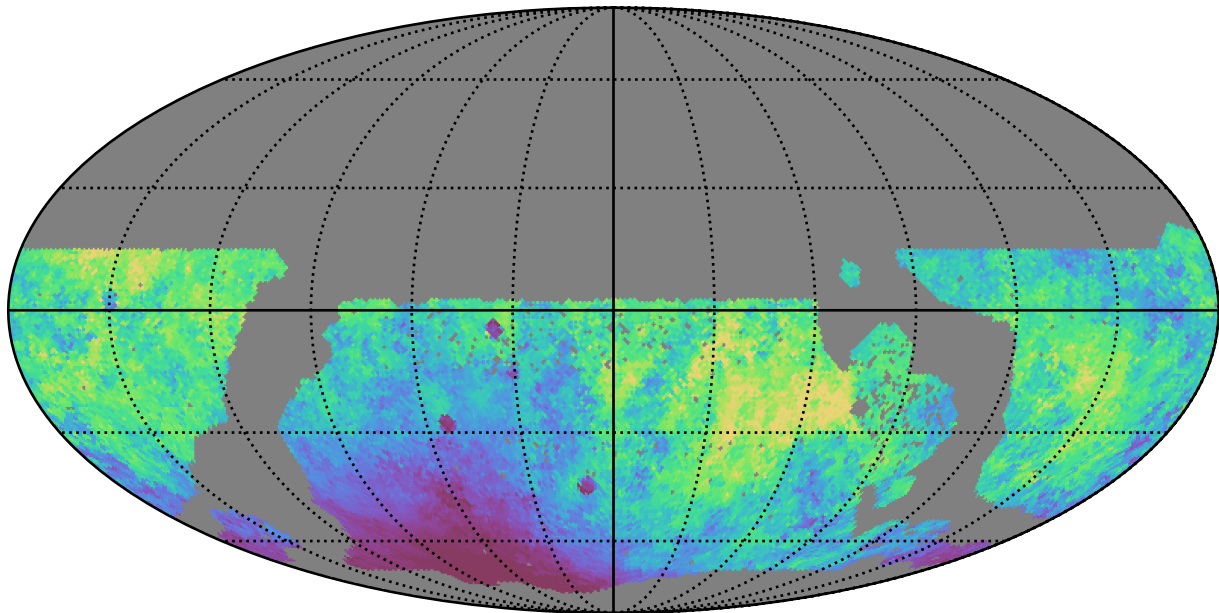
no_magell_roll_v3.4_10yrs WFD r band: Median moonDistance
