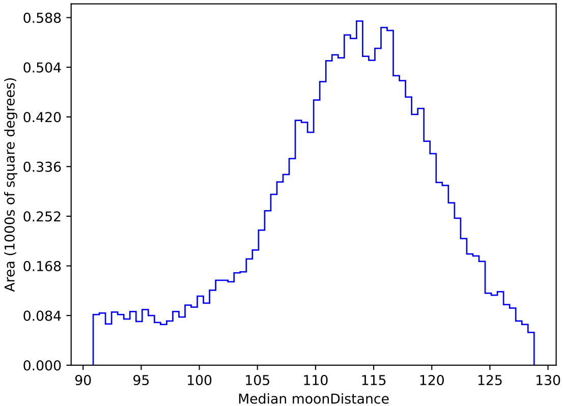
no_magell_roll_v3.4_10yrs WFD r band: Median moonDistance
