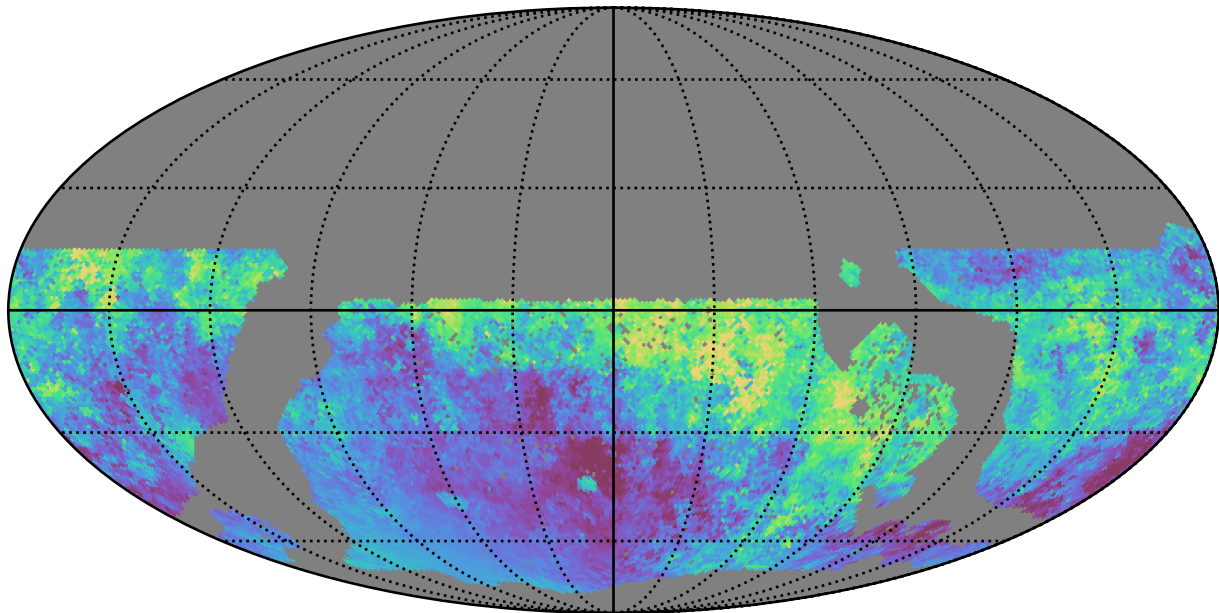
no_magell_roll_v3.4_10yrs WFD i band: Median moonDistance
