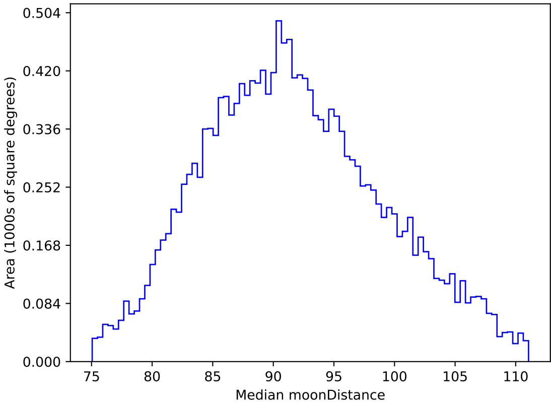
no_magell_roll_v3.4_10yrs WFD i band: Median moonDistance
