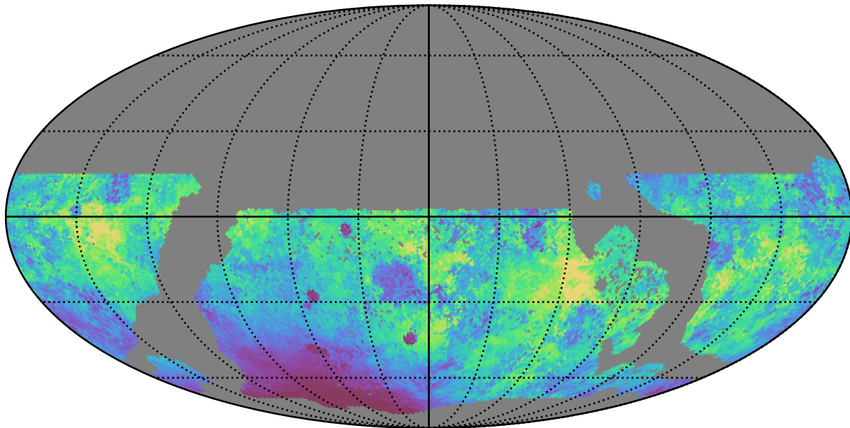
no_magell_roll_v3.4_10yrs WFD g band: Median moonDistance
