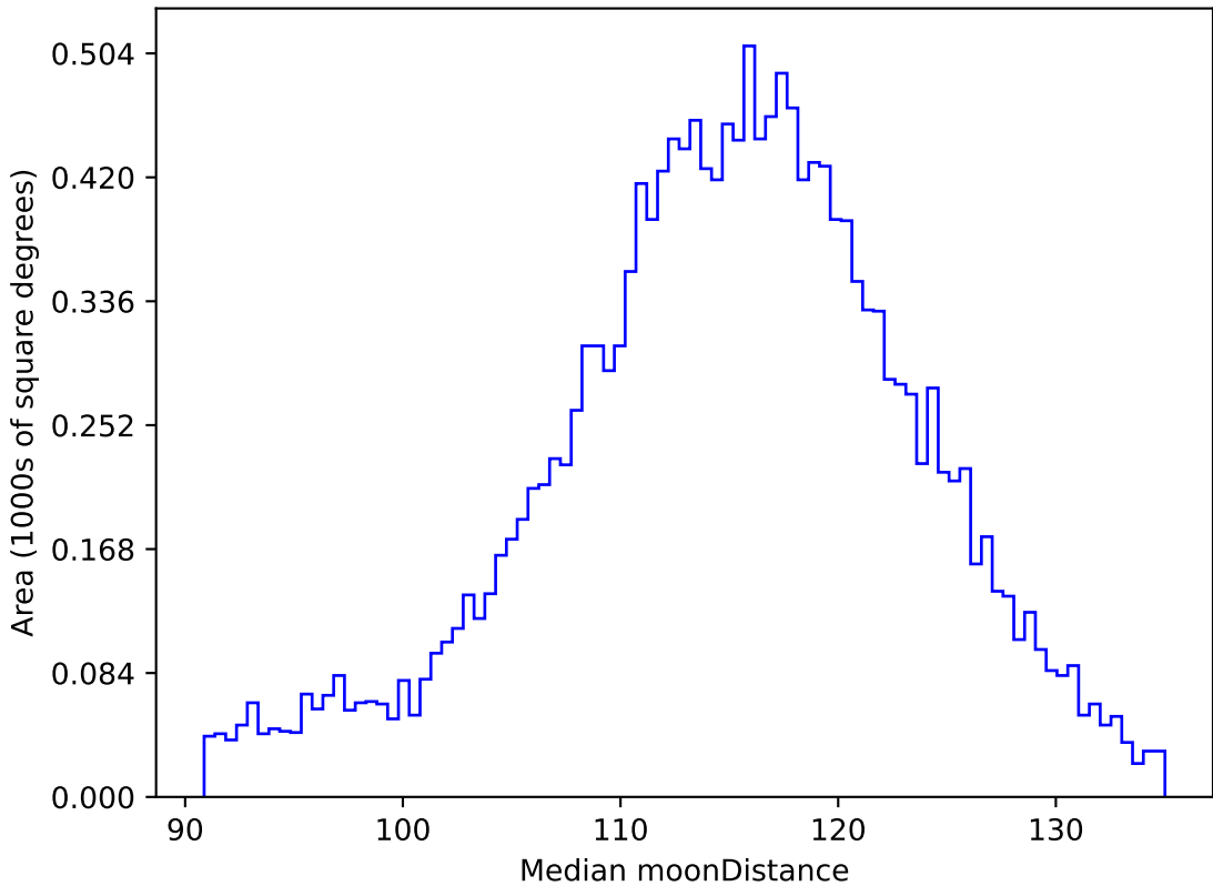
no_magell_roll_v3.4_10yrs WFD g band: Median moonDistance
