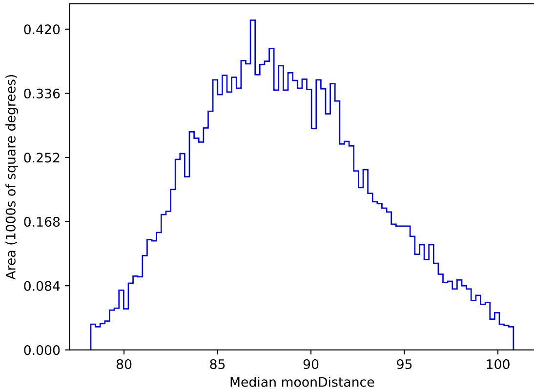
no_magell_roll_v3.4_10yrs WFD all bands: Median moonDistance
