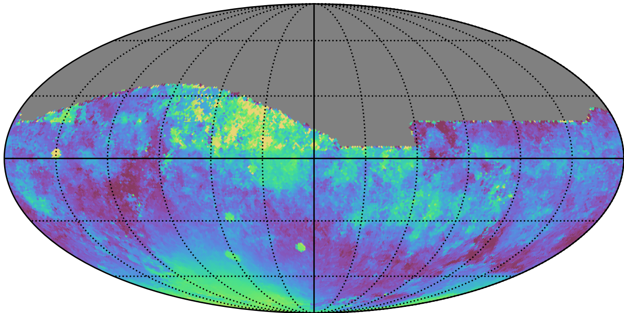
no_magell_roll_v3.4_10yrs All sky z band: Median moonDistance
