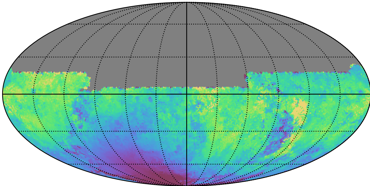
no_magell_roll_v3.4_10yrs All sky u band: Median moonDistance
