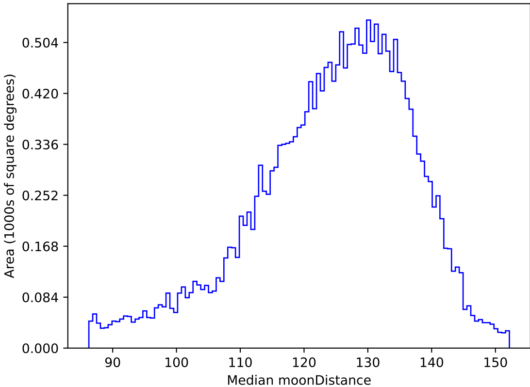
no_magell_roll_v3.4_10yrs All sky u band: Median moonDistance
