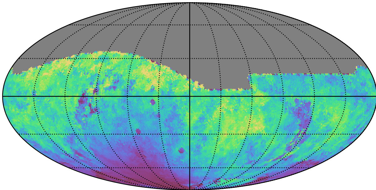
no_magell_roll_v3.4_10yrs All sky r band: Median moonDistance
