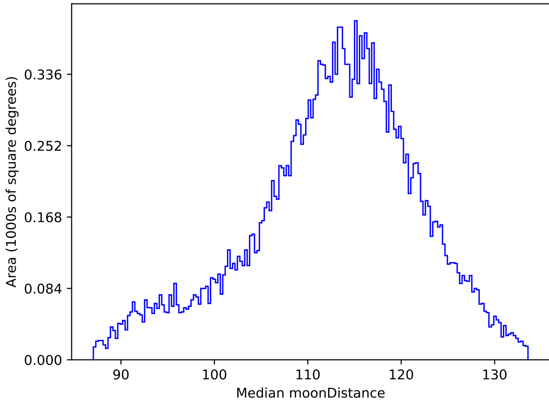
no_magell_roll_v3.4_10yrs All sky r band: Median moonDistance
