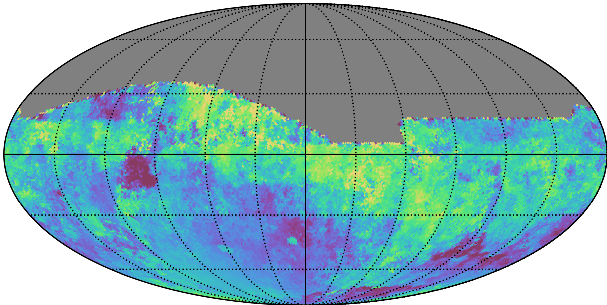
no_magell_roll_v3.4_10yrs All sky i band: Median moonDistance
