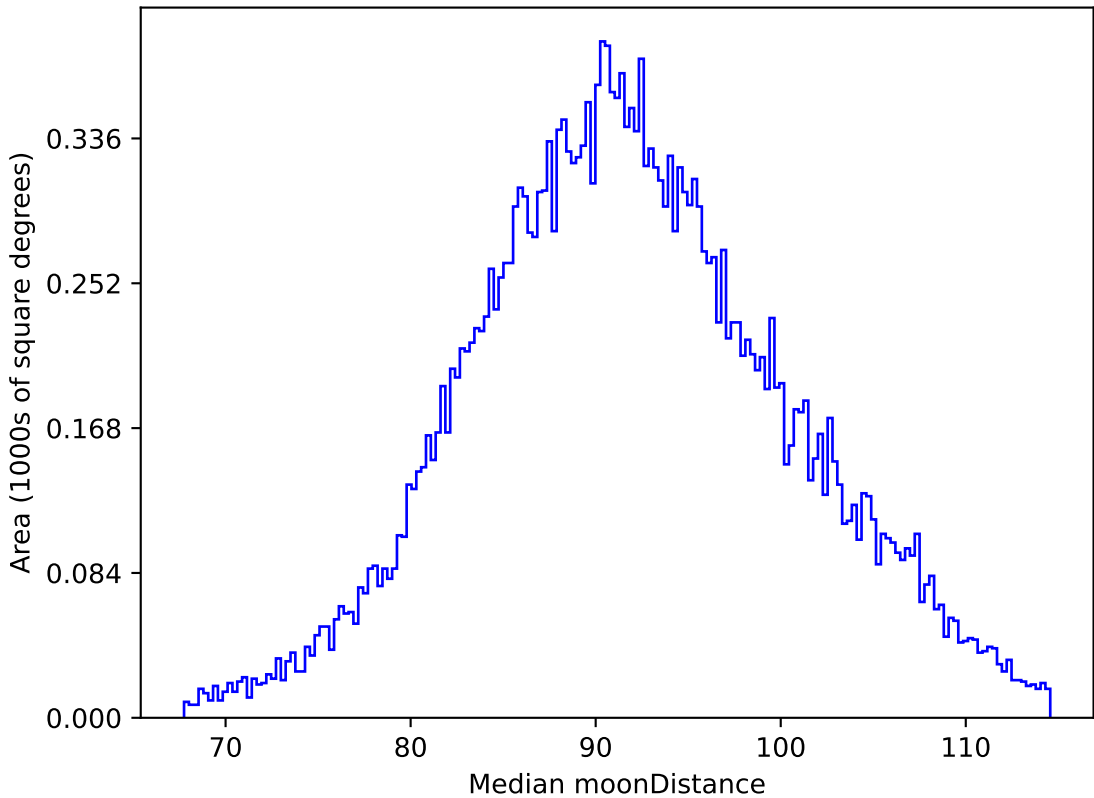
no_magell_roll_v3.4_10yrs All sky i band: Median moonDistance
