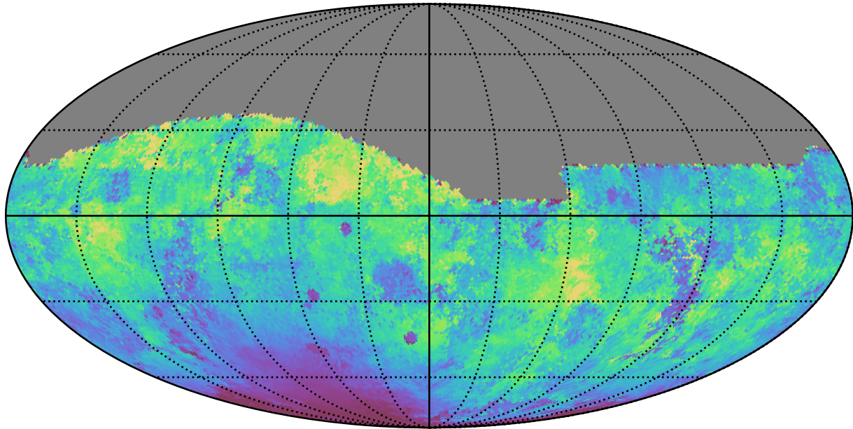
no_magell_roll_v3.4_10yrs All sky g band: Median moonDistance
