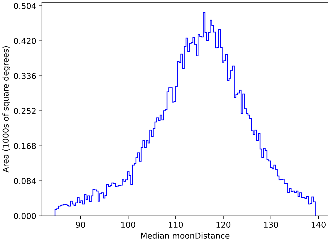
no_magell_roll_v3.4_10yrs All sky g band: Median moonDistance
