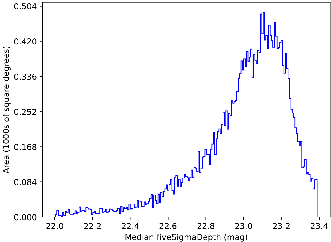
no_magell_roll_v3.4_10yrs Yr 1 z band: Median fiveSigmaDepth
