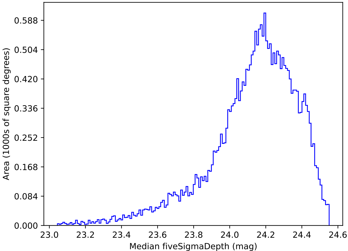
no_magell_roll_v3.4_10yrs Yr 1 r band: Median fiveSigmaDepth
