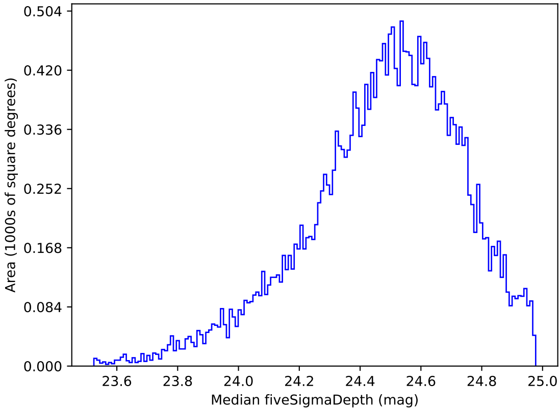
no_magell_roll_v3.4_10yrs Yr 1 g band: Median fiveSigmaDepth
