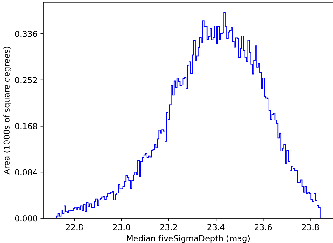
no_magell_roll_v3.4_10yrs Yr 1 all bands: Median fiveSigmaDepth
