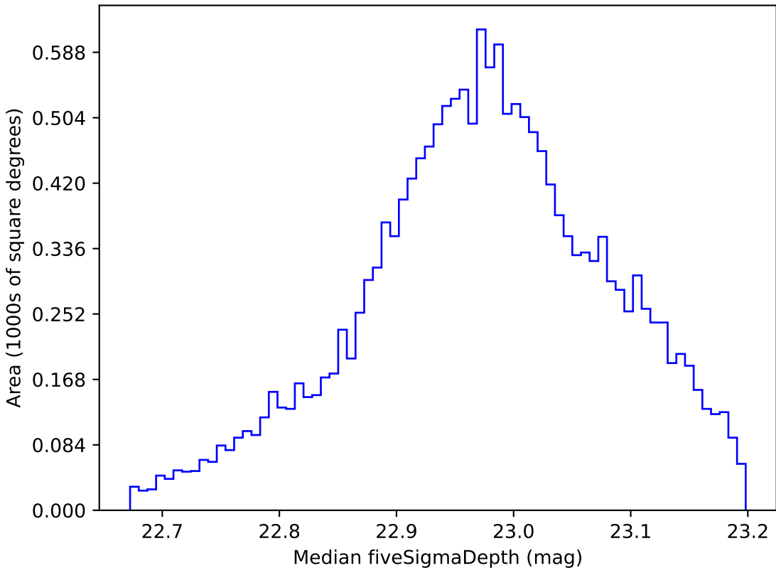
no_magell_roll_v3.4_10yrs WFD z band: Median fiveSigmaDepth
