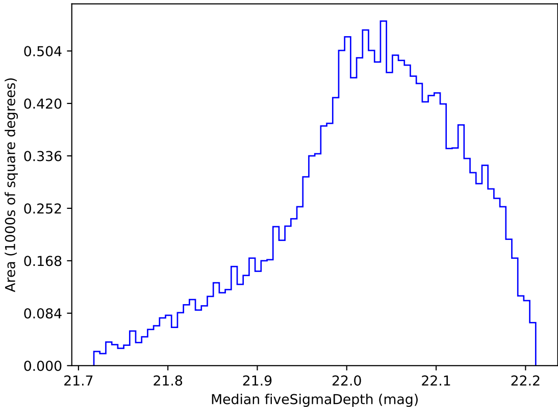
no_magell_roll_v3.4_10yrs WFD y band: Median fiveSigmaDepth
