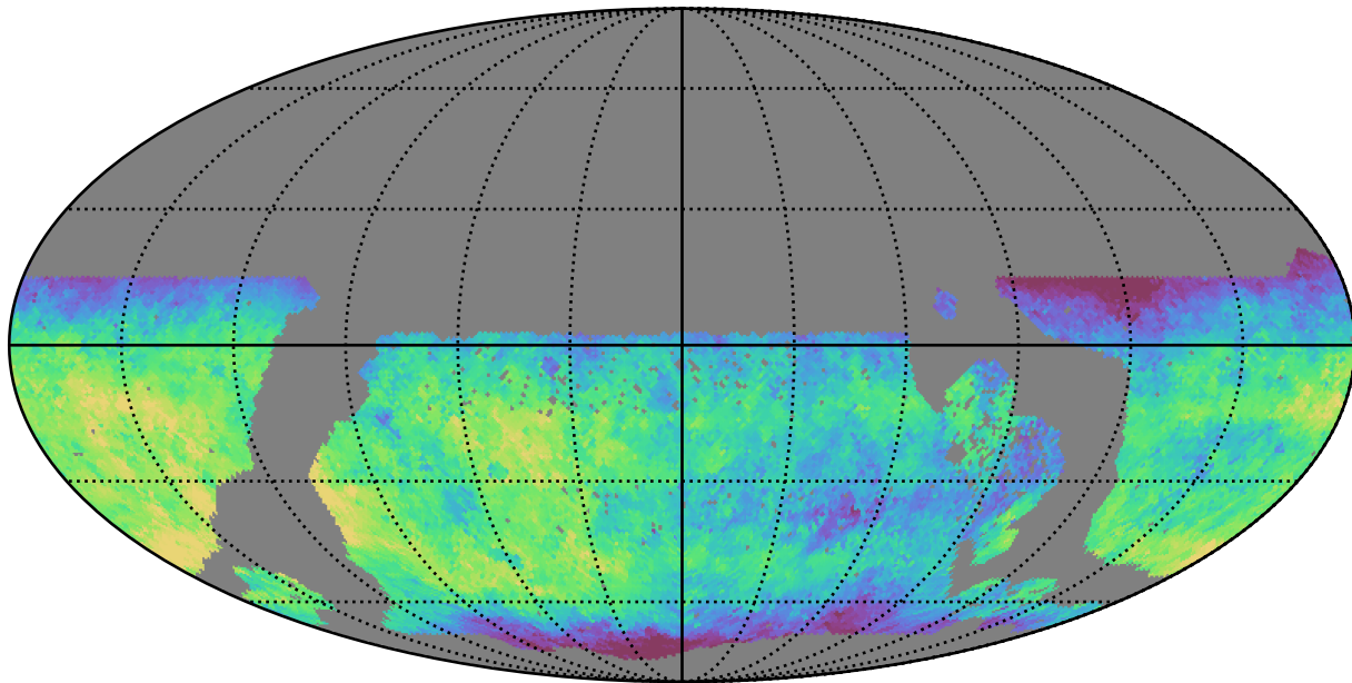
no_magell_roll_v3.4_10yrs WFD u band: Median fiveSigmaDepth
