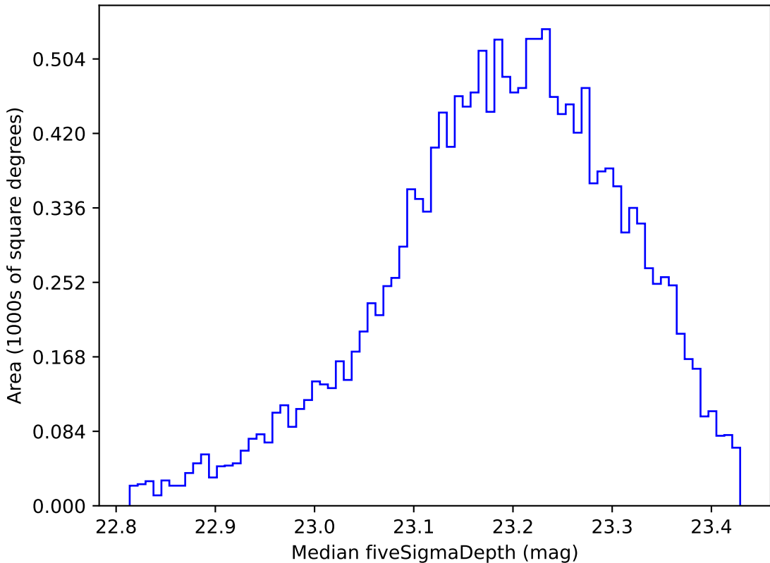
no_magell_roll_v3.4_10yrs WFD u band: Median fiveSigmaDepth
