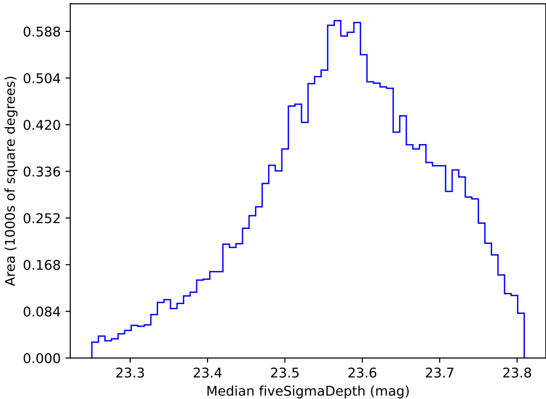
no_magell_roll_v3.4_10yrs WFD i band: Median fiveSigmaDepth
