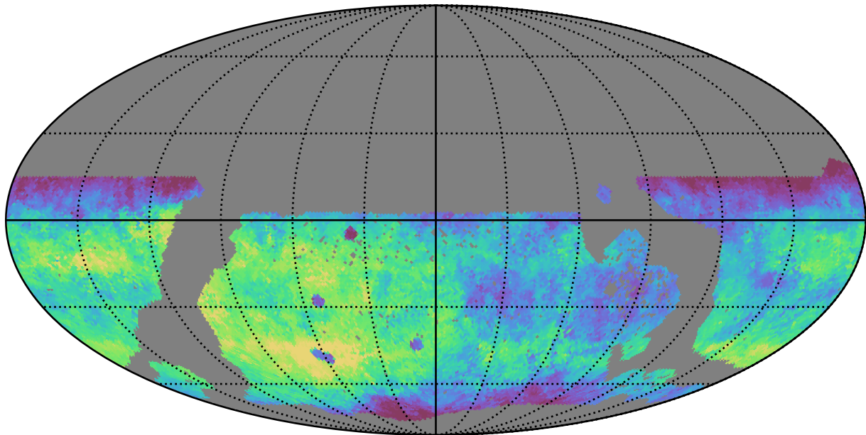
no_magell_roll_v3.4_10yrs WFD g band: Median fiveSigmaDepth
