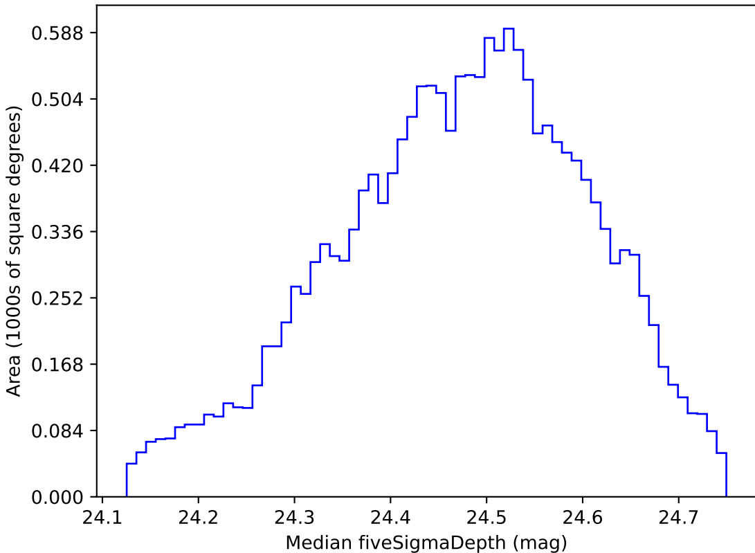
no_magell_roll_v3.4_10yrs WFD g band: Median fiveSigmaDepth
