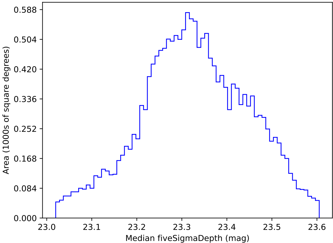
no_magell_roll_v3.4_10yrs WFD all bands: Median fiveSigmaDepth
